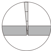
fit-up gap
